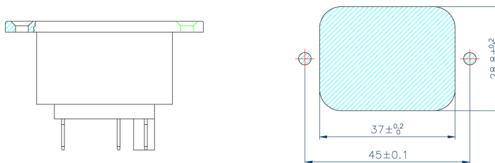
PANEL CUTOUT
