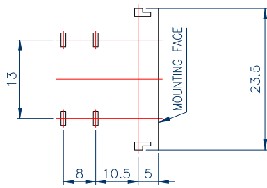
P.C. BOARD MOUNTING HOLD DIMENSION
